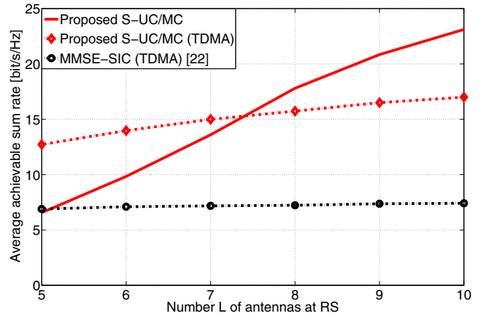
Fig. 8. Average achievable sum rates versus number L of antennas at RS for an average receive SNR= 15dB at RS, G = 2 , N = 4 .
